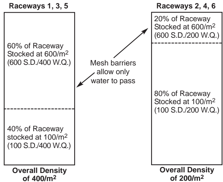
Figure 2. Schematic diagram of the experimental setup designed to separate the effects of shrimp density from water quality.
